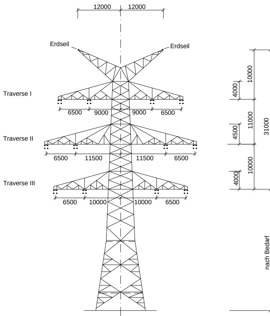
Winkelabspannmast WA140; DD-4-TT-2015.1 Ltg. Nr. 315: Mast-Nr. 58, 59, 62
