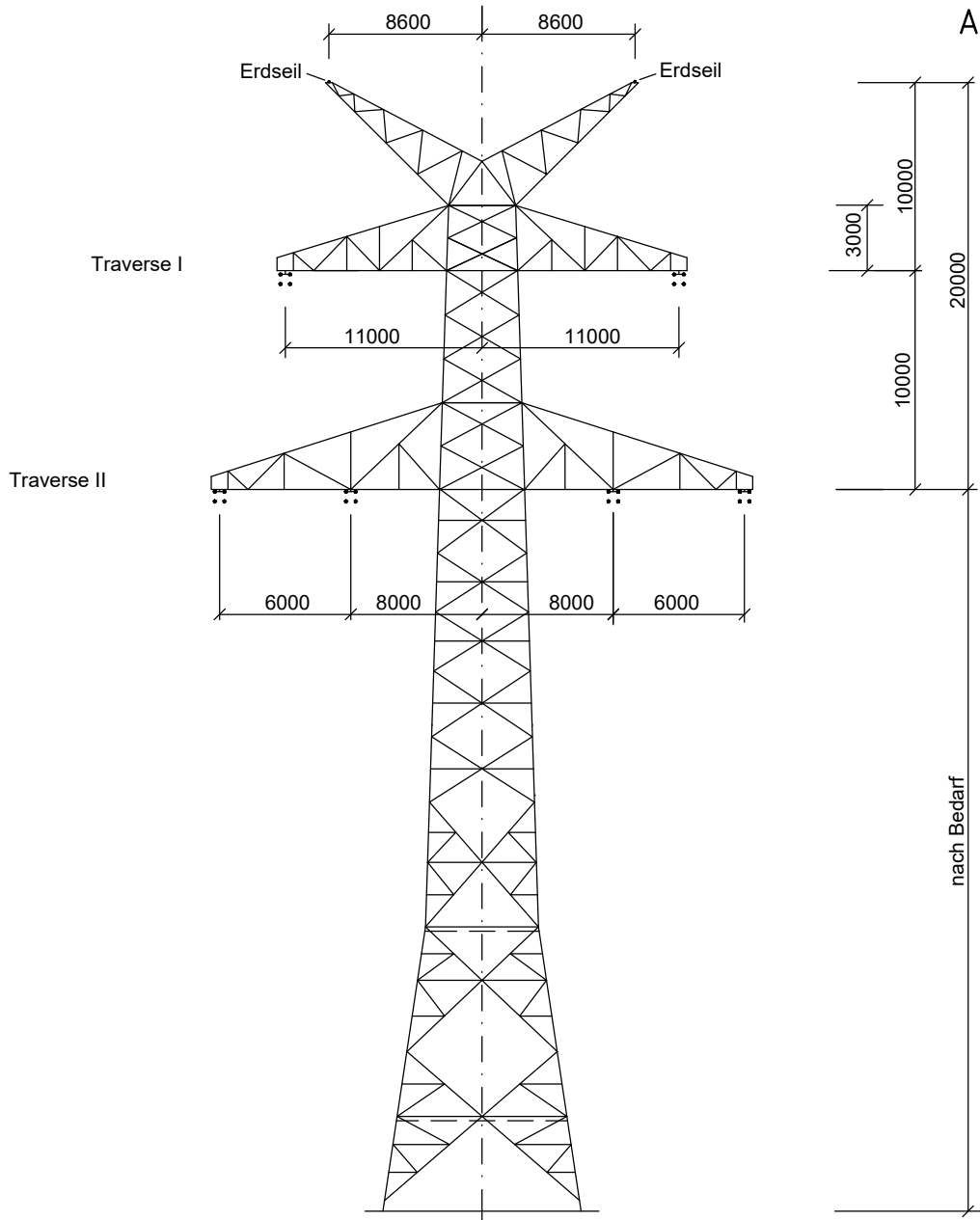
Winkelabspannmast WA160; D-2-D-2015.3 Ltg. Nr. 315: Mast-Nr. 11, 12, 14, 16, 26, 37
