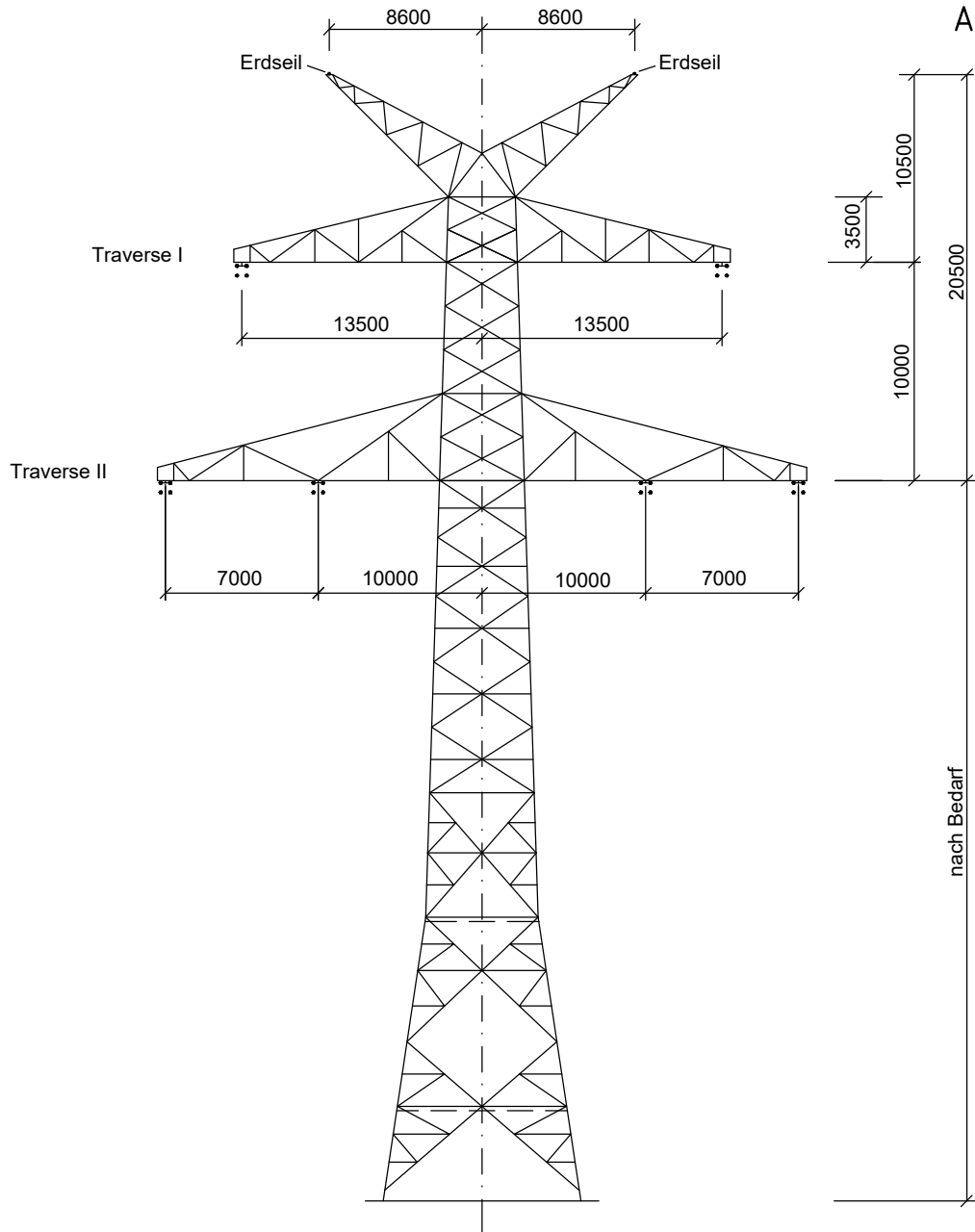
Winkelabspannmast WA120; D-2-D-2015.3 Ltg. Nr. 315: Mast-Nr. 1A, 2, 42, 44, 45, 51
