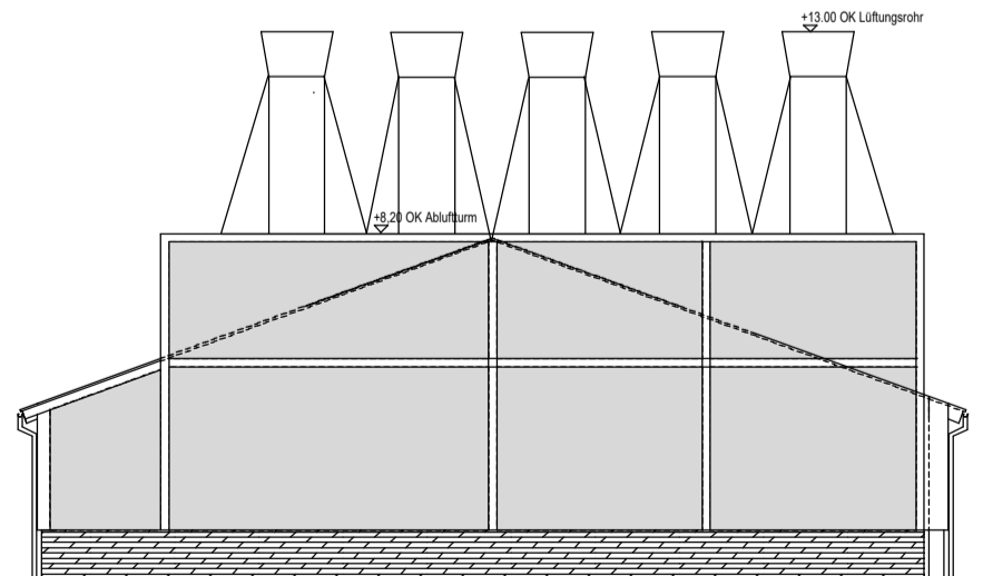
Stall 1
