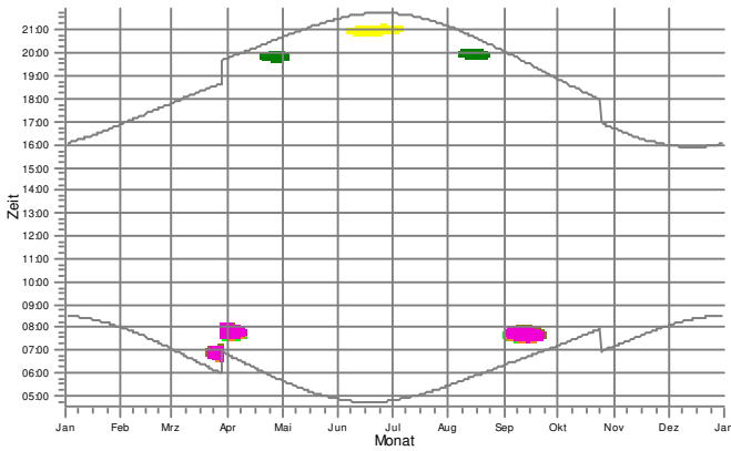
WEA 04: WEA 04 - GE 5.5-158^161m
