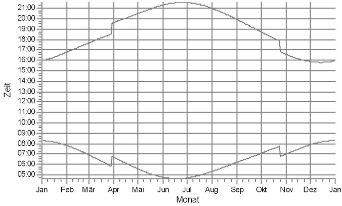
S: IO U Angermünder Straße 21, Felchow, Schatten
