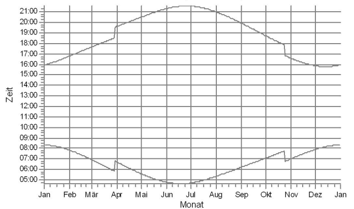
F: IO G Kerkower Straße 6, Dobberzin, Schatten
